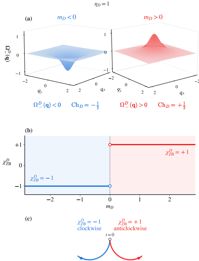
FIG. 1. Relation between the Dirac mass, Berry curvature, and Zitterbewegung chirality near a Dirac point. For a fixed Dirac-point chirality \eta_D = +1 , the sign of the Dirac mass m_D determines the signs of the Berry curvature \Omega_D^D and the local Chern contribution \text{Ch}_D . (a) Berry curvature near the Dirac point for m_D < 0 and m_D > 0 . (b) The Zitterbewegung chirality \chi_{\text{ZB}}^D = \text{sgn}(\text{Ch}_D) changes sign with m_D and is undefined at m_D = 0 , where the gap closes. (c) Schematic Zitterbewegung trajectories illustrating the corresponding change from clockwise to anticlockwise motion.
