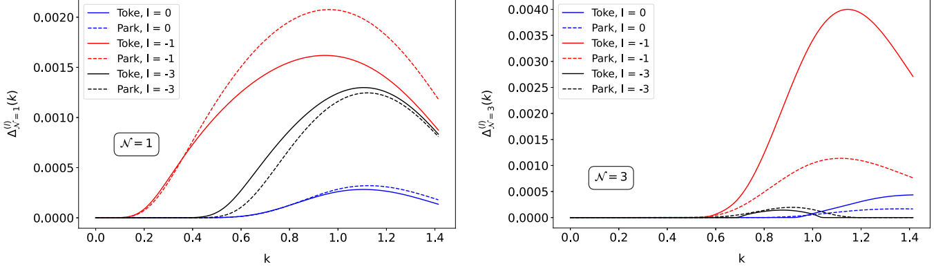
FIG. 2. Self-consistently calculated solutions for \Delta(k) for different pairing channels l in the second ( \mathcal{N}=1 ) (left) and fourth ( \mathcal{N}=3 ) (right) Landau levels (LLs). These results correspond to the Toke and Park interactions.
