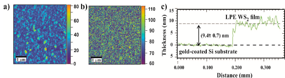
Figure 4. (a) AFM topographic image of the LPE-LS \text{WS}_2 film on the \text{SiO}_2/\text{Si} substrate (image includes a false color bar) of 5 \times 5 \mu\text{m}^2 , (b) phase image of the LPE-LS \text{WS}_2 thin film from the same area (image includes a false color bar) showing more contrast around the edges of the nanoflakes, and (c) height profile of the LPE-LS \text{WS}_2 film/Au-coated Si substrate performed by the optical profilometer (measurement started from the gold-coated Si substrate).
