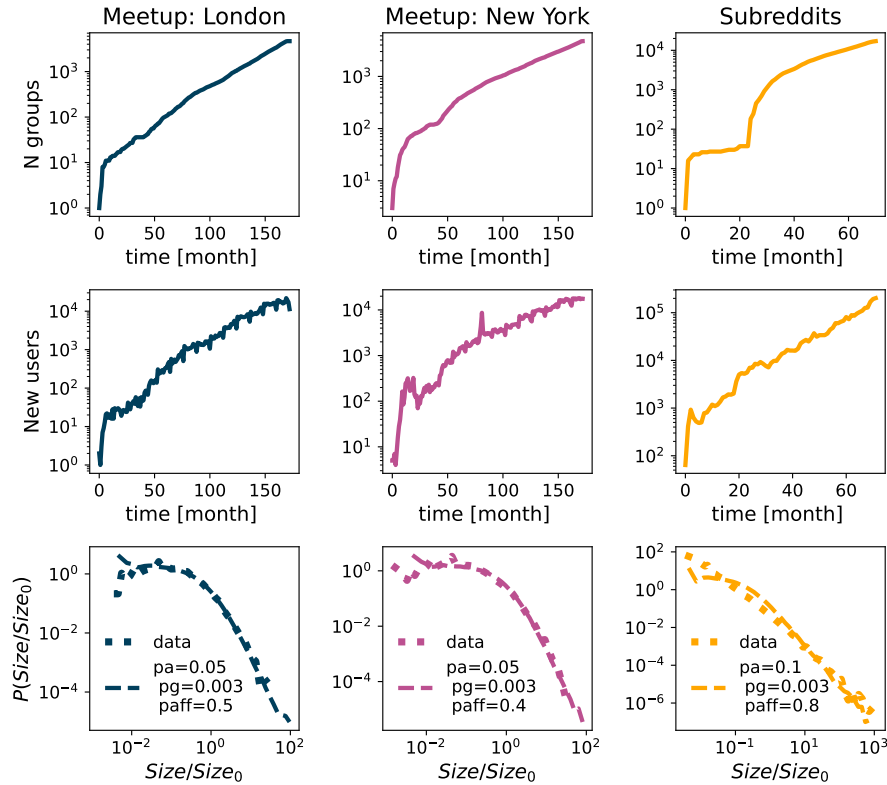
Fig. 1. The number of groups over time (top panel), the time series of new users (middle panel) and the distribution of group sizes (bottom panel - dotted line) at the end of the observed period for Meetup groups in London, New York and Subreddits. The number of groups and new users grows exponentially, while the distributions of group sizes follow log-normal distribution in all systems. Using groups growth model we are able to simulate groups sizes distributions (bottom panel - dashed lines). At each time step new users arrive to the system, following time series of the new users (middle panel). The model parameters: p_a probability that user is active; probability that user creates new group p_g ; and probability that user has preference toward friend's groups, p_{aff} , are approximated from the data.
