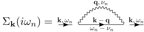
FIG. S6. Feynman diagrams of the self-energy in the Migdal approximation
