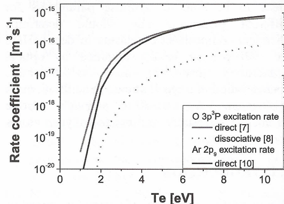
Fig. 2 Rate coefficients for direct excitation of Ar and O atoms (full lines) and dissociative excitation of O (dashed line)
