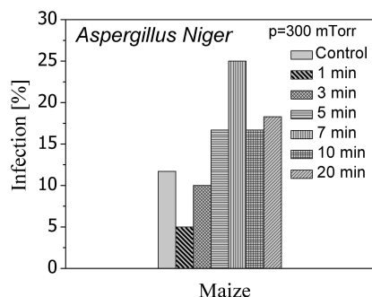
Fig. 4. Infection of maize after plasma treatment in asymmetrical CCP discharge. Control represents untreated seeds. Feeding gas was air at a pressure of p = 300 mTorr. Power given by RF power supply was 200 W
