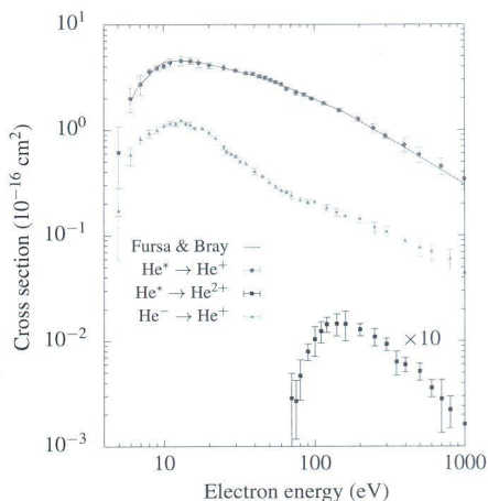
Figure 1. Cross sections for electron-impact single and double ionization of He(1s2s 3 S) and double ionization of He - .
