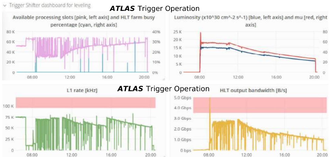
Figure 18. An example of a P-BEAST dashboard as used by the shifters during 2017 operation. The HLT farm availability (top left), the luminosity and the pile-up, ‘ \mu ’ (top right), the total L1 accept rate (bottom left), and the total HLT output bandwidth (bottom right) are shown.
