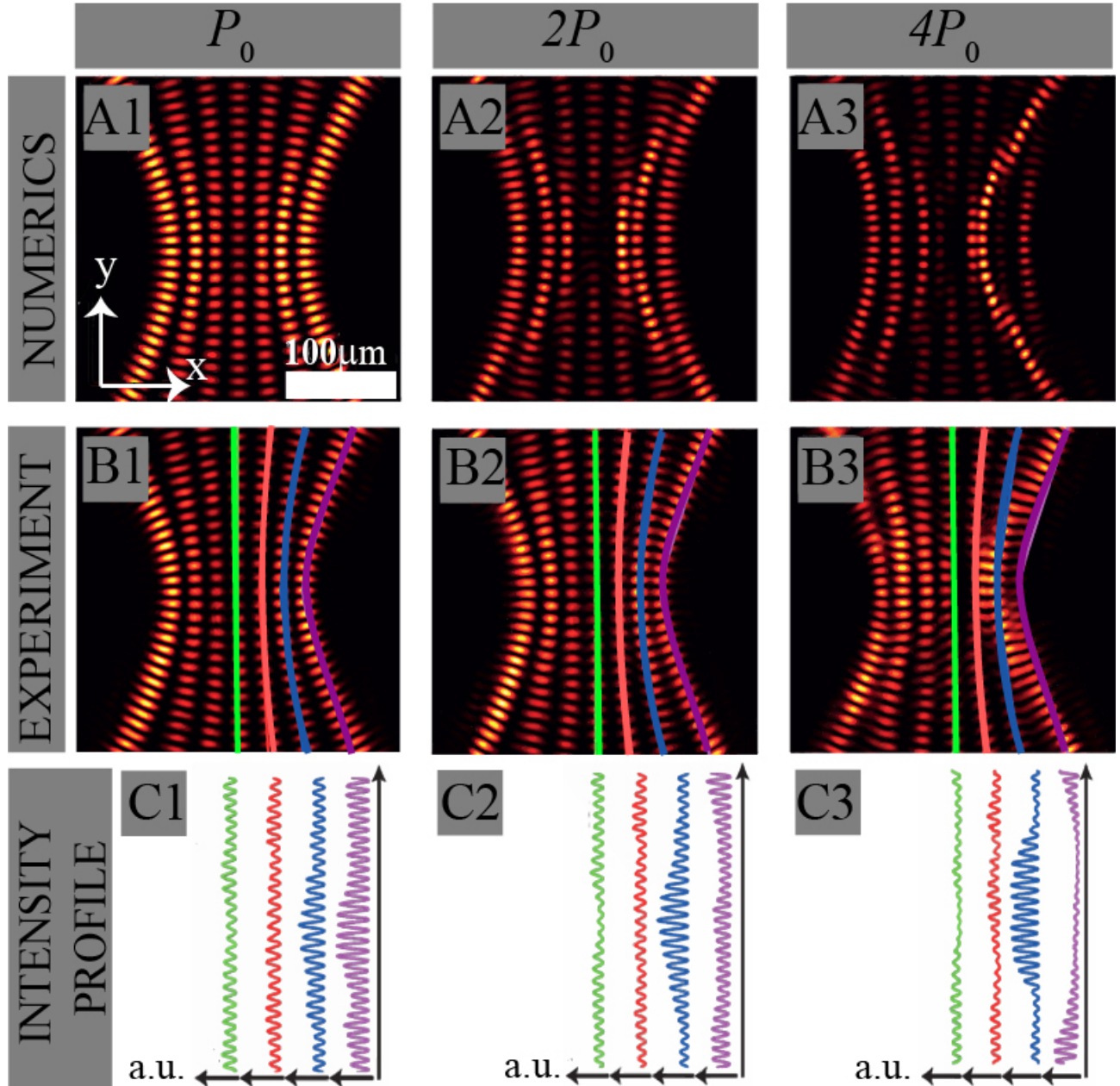
Figure 6.4: Switching discrete diffraction on curved paths based on the self-action of sixth-order even Mathieu beam: (A) simulated and (B) experimentally observed transverse intensity distributions at the crystal's back face. (C) Intensity profiles along the hyperbolic waveguide layers indicated in (B). P_0 = 10\mu\text{W} .
