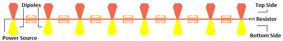
Fig. 4 – Layout of the antenna array.
