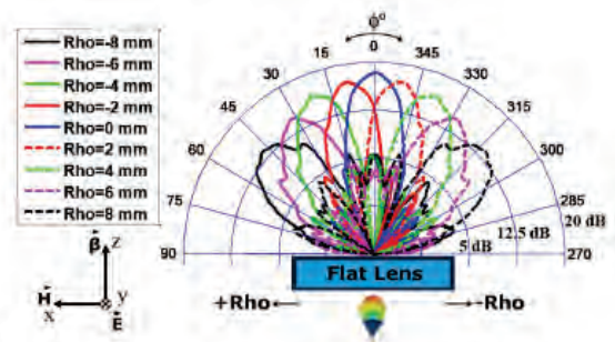
Fig. 8. Measured H-plane radiation patterns at 60 GHz for the different values of feeding positions, Rho (-8 mm to 8 mm) (after [15]).
