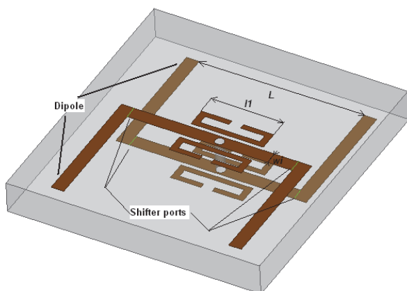
Fig. 2. Layout of SRR phase shifter with relevant dimensions: l_1 = 7.2 \text{ mm} , w_1 = 0.4 \text{ mm} , L = 25 \text{ mm}
