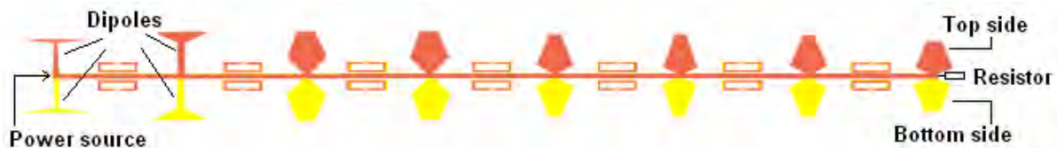
Fig. 3. Antenna array with pentagonal dipoles and resistor termination.
