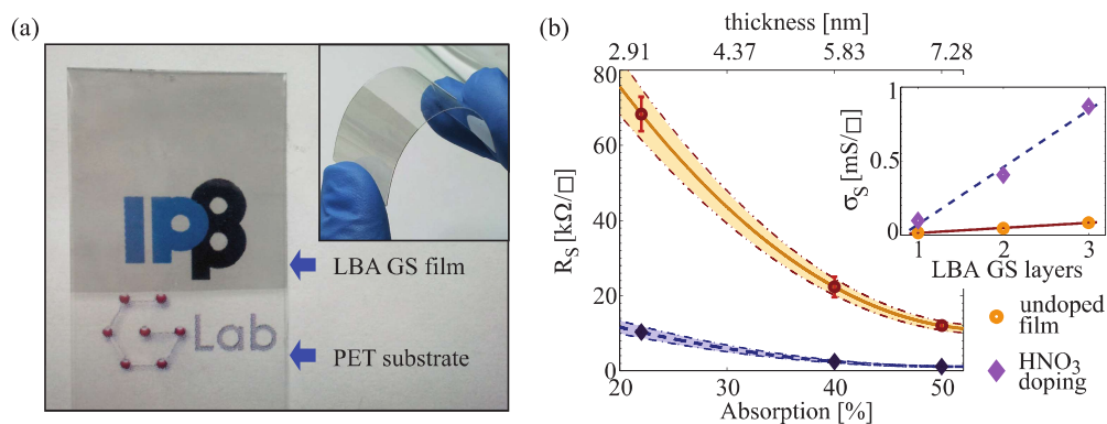
FIGURE 1. (a) 2 \times 2 cm 2 LBA graphene sheet (GS) film on a polyethylene terephthalate (PET) substrate. (b) The sheet resistance ( R_S ) and sheet conductivity ( \sigma_S ) of stacked LBA GS layers, prior and after chemical doping.
