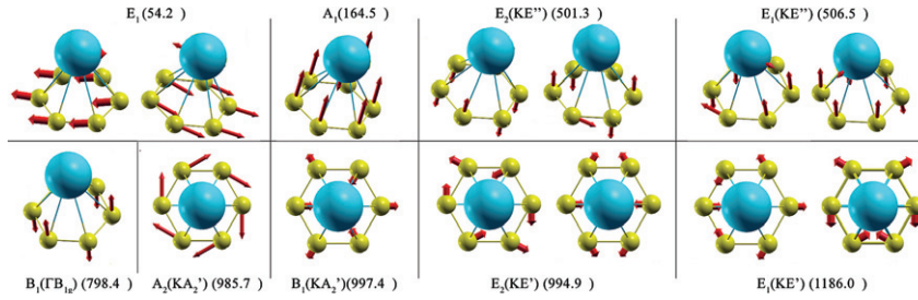
Fig. 3: (Color online) Vibrational frequencies (in wave numbers) and displacement patterns for the monolayer BaC 6 -mono. The modes of graphene with a similar displacement pattern are denoted in parentheses.
