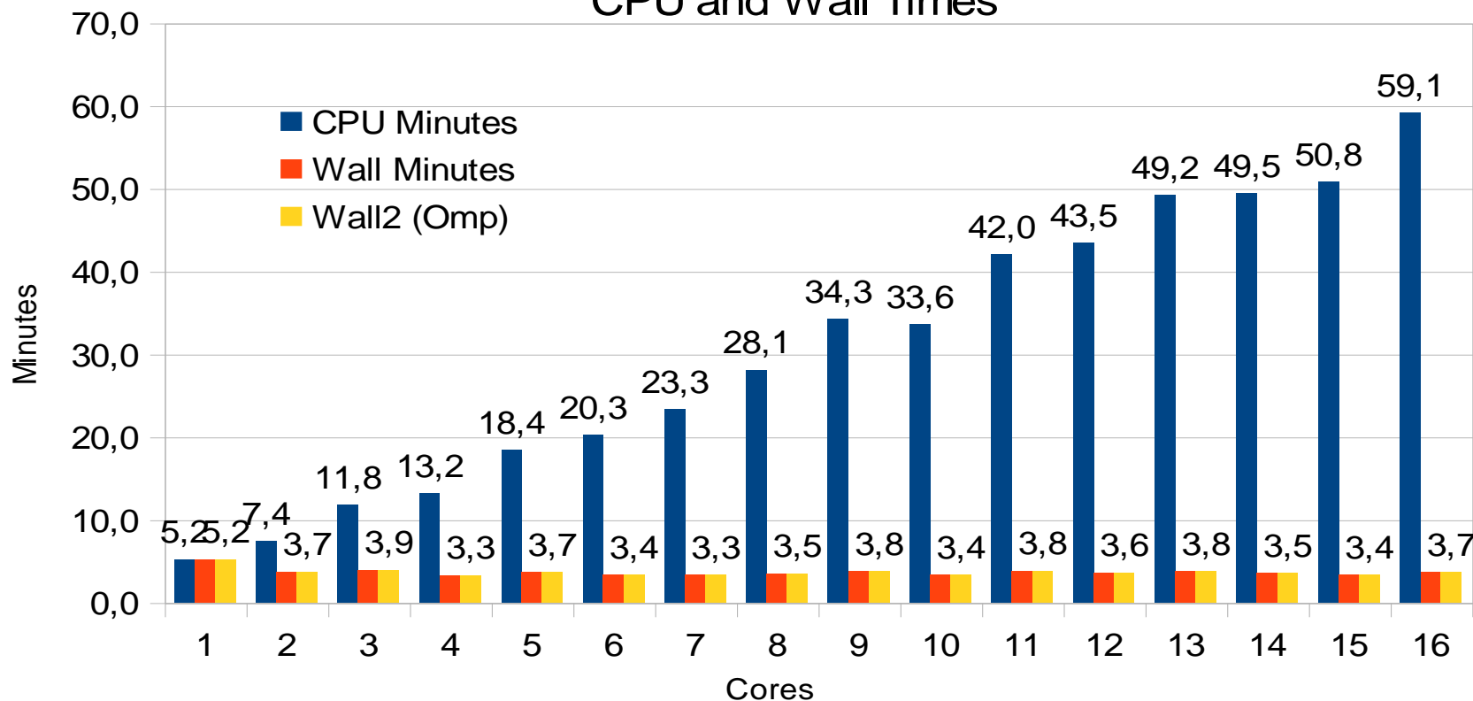
AMR_PAR 128x128x128 5 layers,HPCG cluster CPU and Wall Times
