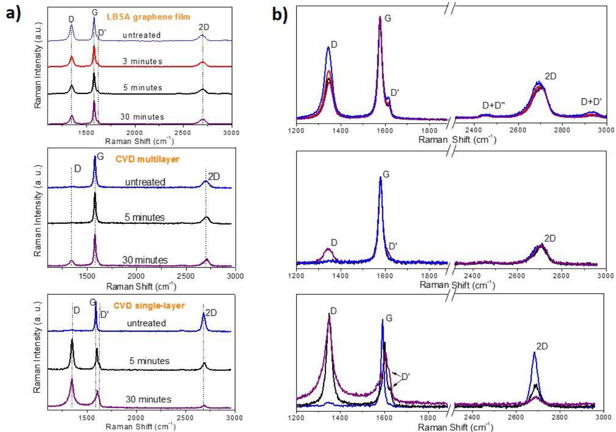
Fig. S1 (a) Raman spectra of the LBSA, CVD-grown multilayer and CVD-grown single-layer graphene films as a function of UVO exposure time, (b) Close-up view of the main bands of (a).
