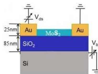
Figure 1: Schematic “cross-sectional” view of the device
