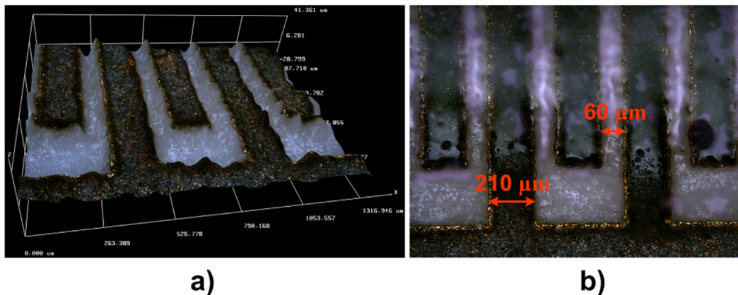
Fig. 3. a) A 3D image of the part of interdigitated electrodes before electrolyte deposition and b) a 2D image of the part of interdigitated electrodes after electrolyte deposition. Images were obtained by Huvitz HRM 300 profilometer.
