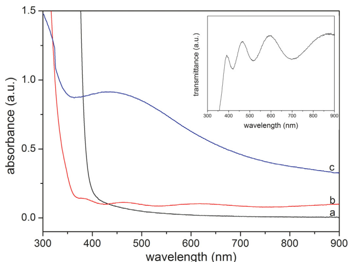
Fig. 2. Absorption spectra of precursor 4.5 nm TiO 2 colloid (a), nanocrystalline TiO 2 film (b), and photochemically deposited metallic silver on nanocrystalline TiO 2 film (c). Inset shows transmission spectrum of nanocrystalline TiO 2 film with interference fringes.
