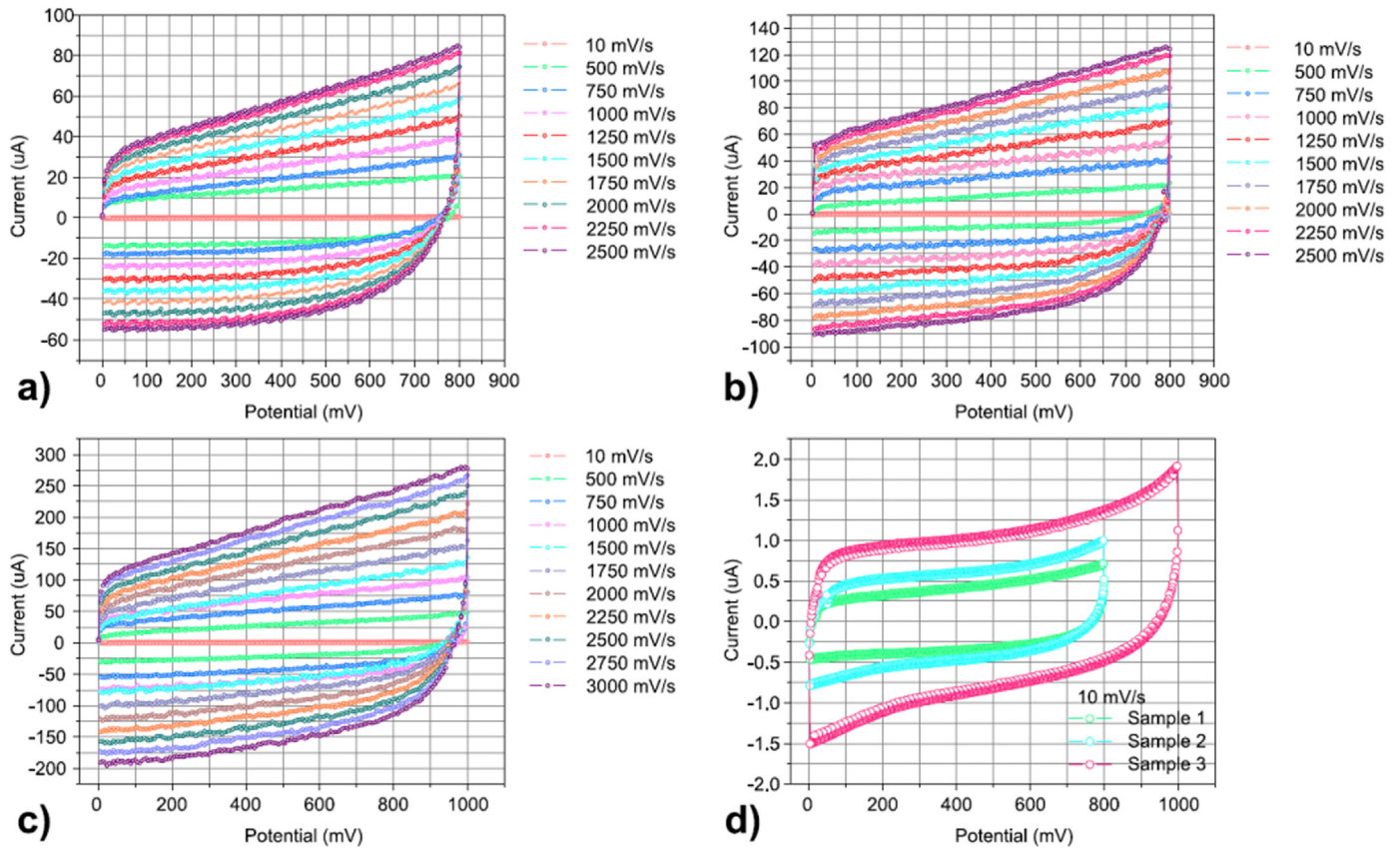
Fig. 4. Electrochemical properties of micro-supercapacitors a) Sample 1, b) Sample 2, c) Sample 3 and d) Comparison of cyclic voltammograms for Sample 1, Sample 2 and Sample 3 at 10 mV/s.
