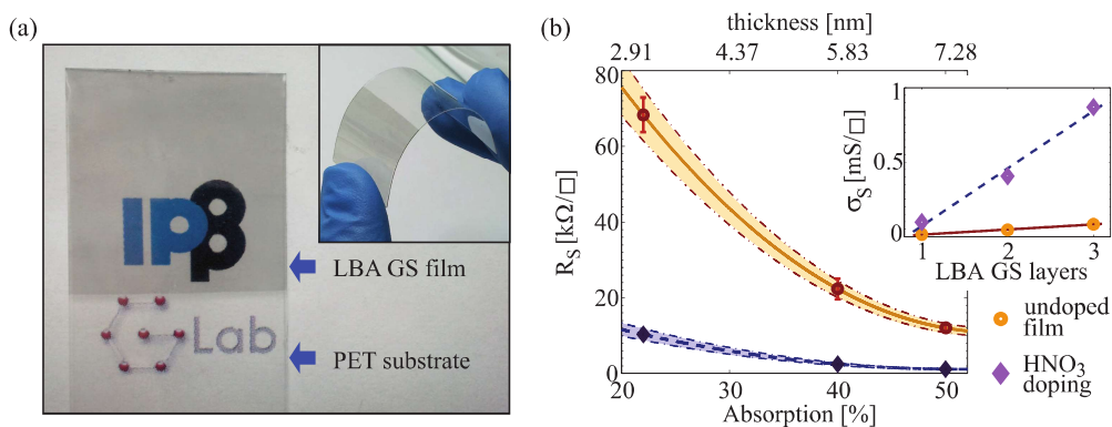
FIGURE 1. (a) 2 \times 2 \text{ cm}^2 LBA graphene sheet (GS) film on a polyethylene terephthalate (PET) substrate. (b) The sheet resistance ( R_S ) and sheet conductivity ( \sigma_S ) of stacked LBA GS layers, prior and after chemical doping.
