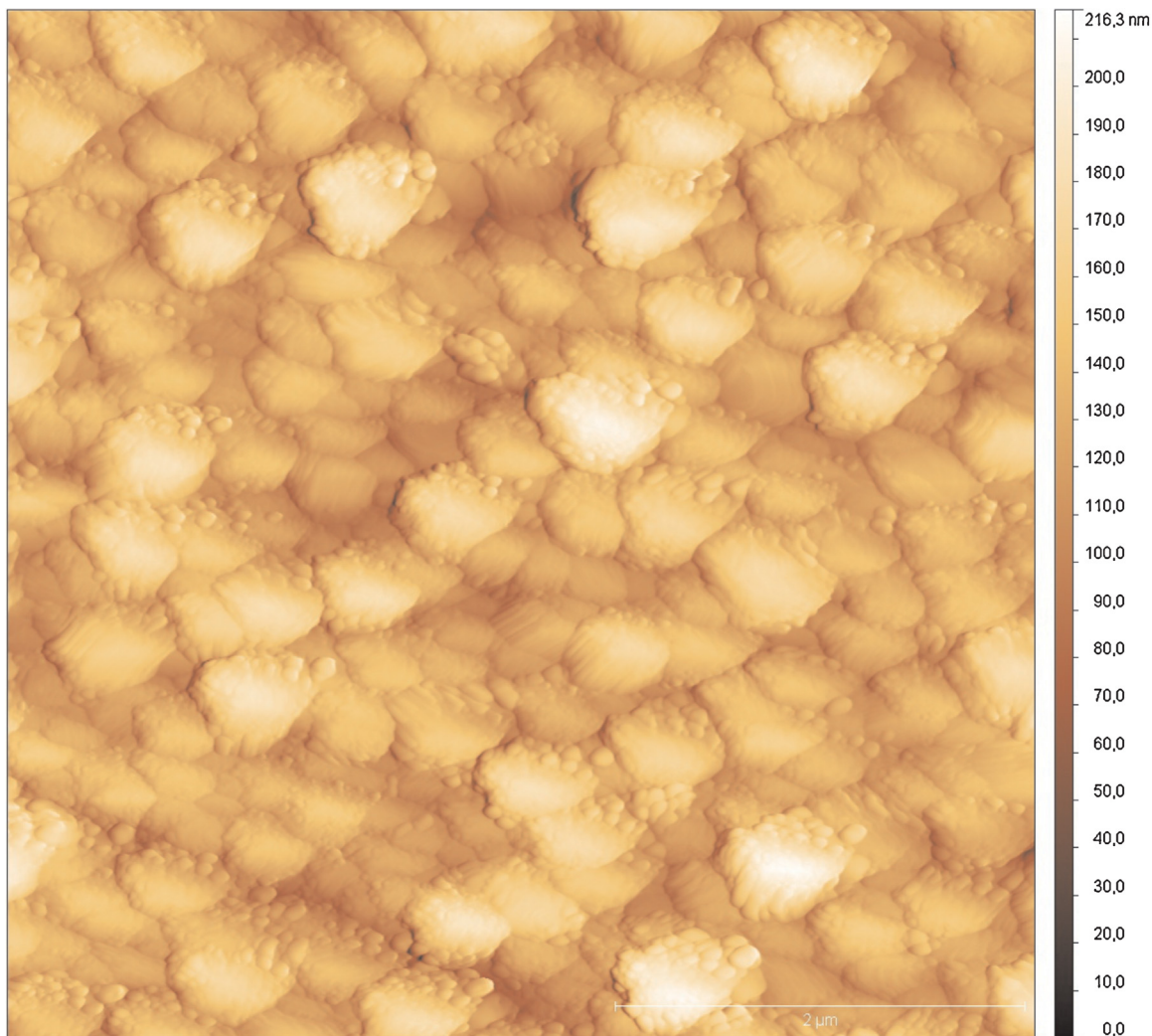
Fig. 3. Typical AFM image of silver grains on the surface of nanocrystalline TiO 2 film.
