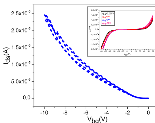
Figure 2: Room-temperature transfer characteristics with 100 mV applied bias voltage, and output characteristics Ids-Vds measured for different gate voltages (inset).
