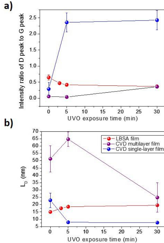
Fig. S2 (a) The D/G intensity ratio of the LBSA, CVD-grown multilayer and CVD-grown single-layer graphene films as a function of UVO exposure time. The D/G ratio is calculated from integrated peak areas. (b) Interdefect distance of the corresponding graphene films as a function of UVO exposure time. The error bar represents the standard deviation of five measurements.
