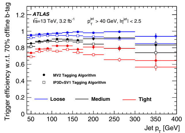
Fig. 46 b -jet trigger efficiency as a function of jet p_T for the loose ( blue ), medium ( black ) and tight ( red ) operating points. The open squares show the trigger efficiency using the IP3D+SV1 b -tagging algorithm. The closed circles show the trigger efficiency for the corresponding MV2 b -tagging algorithm working points. The efficiencies are measured in a pure sample of b -jets selected in t\bar{t} events and are computed with respect to jets identified by the 70% working point of the offline MV2c20 b -tagging algorithm
