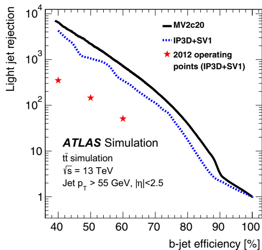
Fig. 45 The expected performance of the MV2c20 trigger tagger ( solid black line ) in terms of light-jet rejection is shown together with the expected performance of the IP3D+SV1 trigger tagger in Run 2 ( dashed blue line ) and its actual performance achieved during Run 1 ( red stars )
