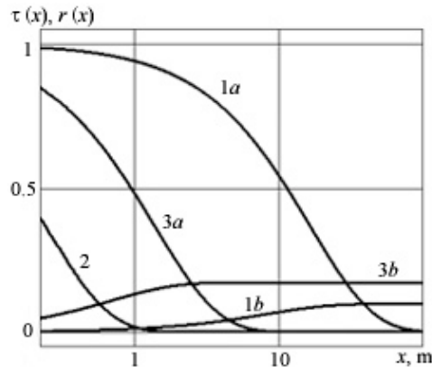
FIGURE 2. Plots of theoretically simulated transparency \tau(x) (lines 1a, 2, 3a) and volumetric reflectance r(x) (lines 1b, 3b) vs seawater depth x (logarithmic scale) for penetrating solar radiation (with the model or experimental albedo A ) for: • natural seawater (NW) for different attenuation coefficients within the following spectral ranges [6, 7]: a) line 1a, 1b – in the blue-green region from \sim 0.3 \mu\text{m} to \sim 0.6 \mu\text{m} at experimental A \sim 10\% caused model volumetric absorption \kappa_{NW} = 0.050 \text{ m}^{-1} and scattering \sigma_{NW} = 0.01 \text{ m}^{-1} coefficients; b) line 2 – in red and near IR regions from \sim 0.6 \mu\text{m} to \sim 2.5 \mu\text{m} with model surface reflectance R_S \sim 2\% and spectrally averaged model absorption coefficient \kappa_{IR} = 5 \text{ m}^{-1} with negligible scattering; • oil-polluted seawater (WOE) with model transparency \tau(x) (line 3a) and reflectance r(x) (line 3b), A = 17\% , \kappa_{WOE} = 0.50 \text{ m}^{-1} , \sigma_{WOE} = 0.25 \text{ m}^{-1} [6, 7].
