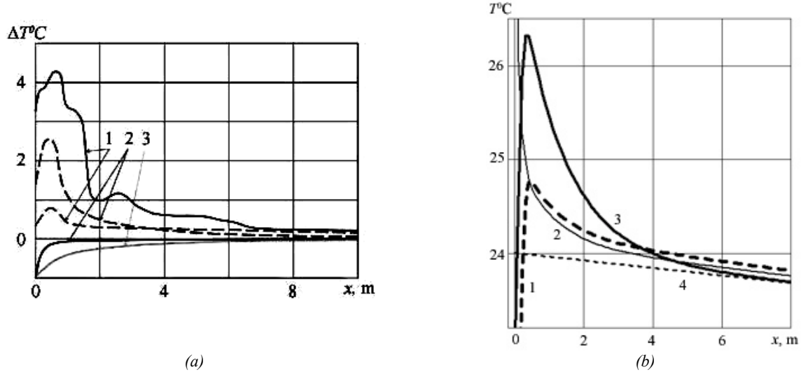
FIGURE 1. Experimental (a) and calculated (b) temperature fields inside subsurface natural and oil-polluted seawaters.
